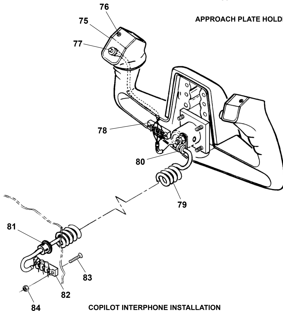
CONTROL WHEEL AND SWITCHES INSTALLATION Figure 02. (Sheet 2)
