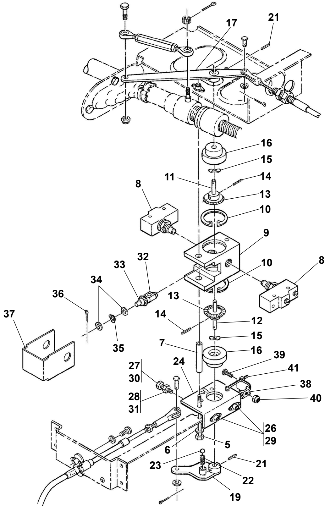
FLAP ACTUATOR SWITCH ASSEMBLY Figure 03. (Sheet 1)
