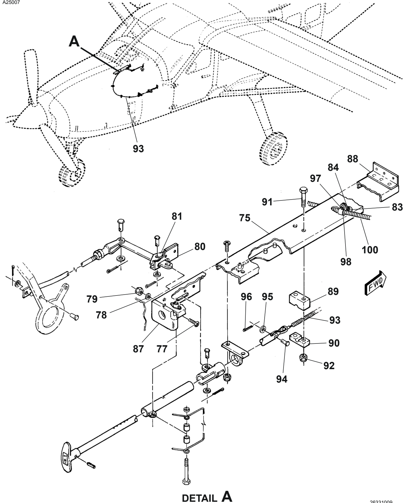
RUDDER CONTROL LOCK INSTALLATION Figure 01. (Sheet 2)
