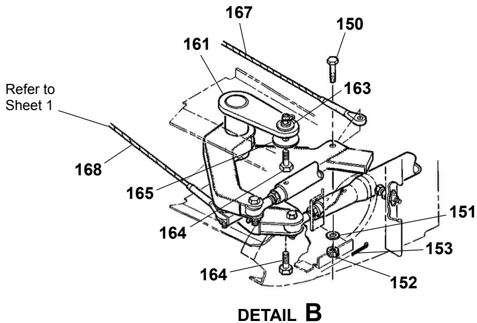
AILERON AND SPOILER CONTROL SYSTEM Figure 02. (Sheet 3)
