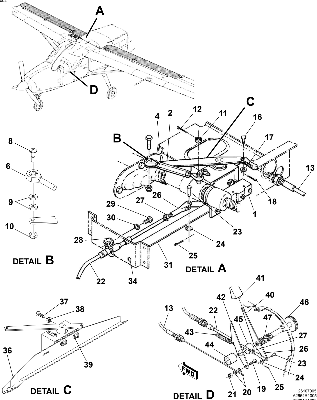
FLAP INDICATOR INSTALLATION Figure 02. (Sheet 1)
