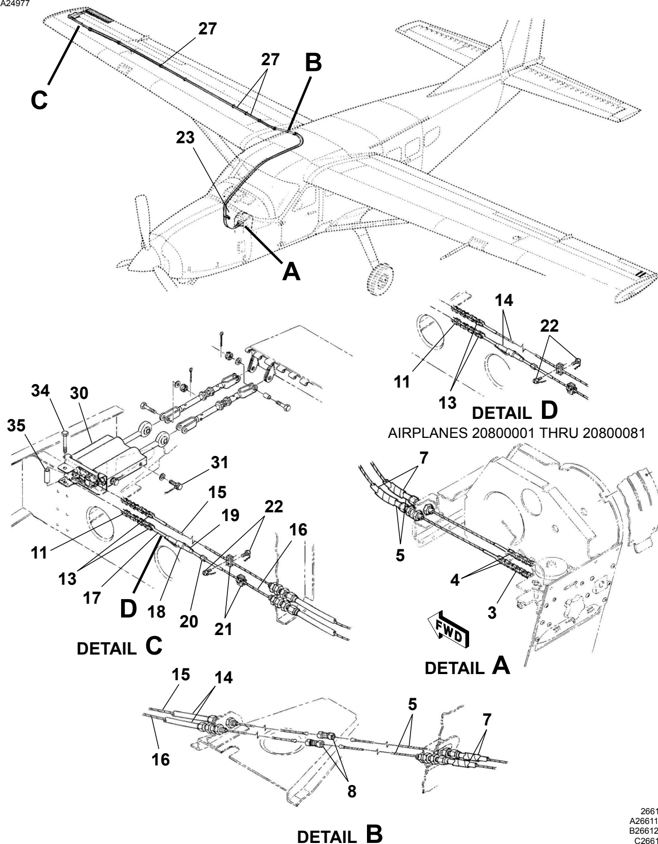
AILERON TRIM CONTROL SYSTEM Figure 01. (Sheet 1)
