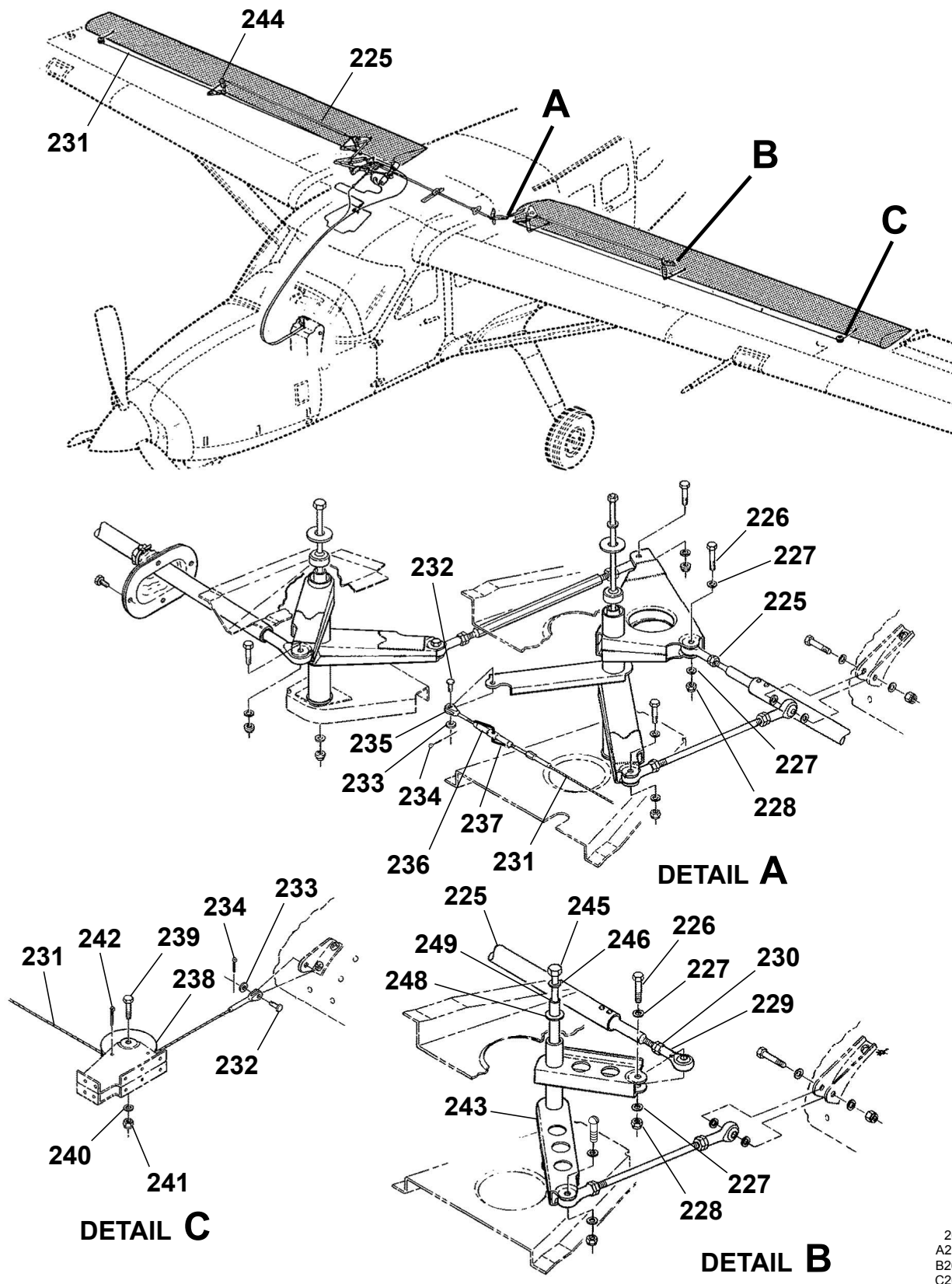
FLAP CONTROL SYSTEM - WING Figure 04. (Sheet 4)
