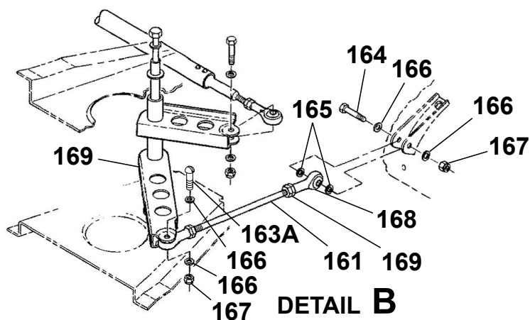
FLAP CONTROL SYSTEM - WING Figure 04. (Sheet 3)
