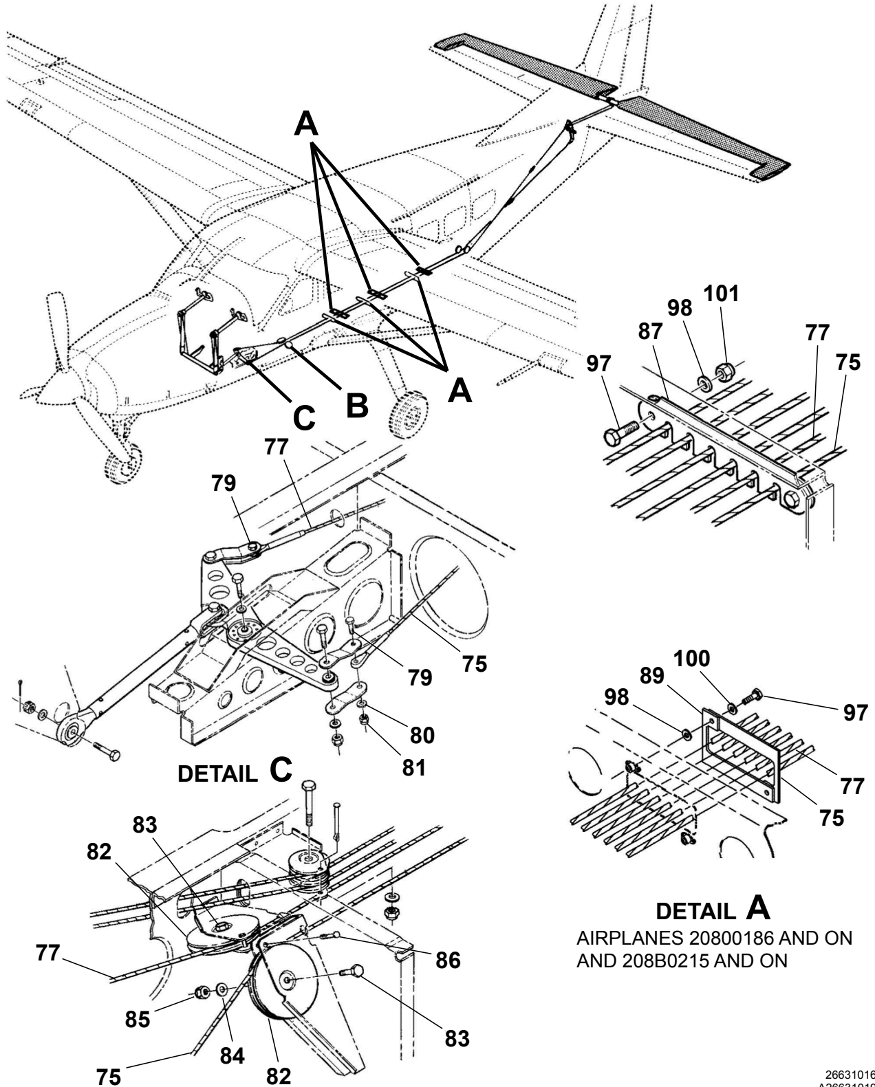
ELEVATOR CONTROL SYSTEM Figure 01. (Sheet 2)
