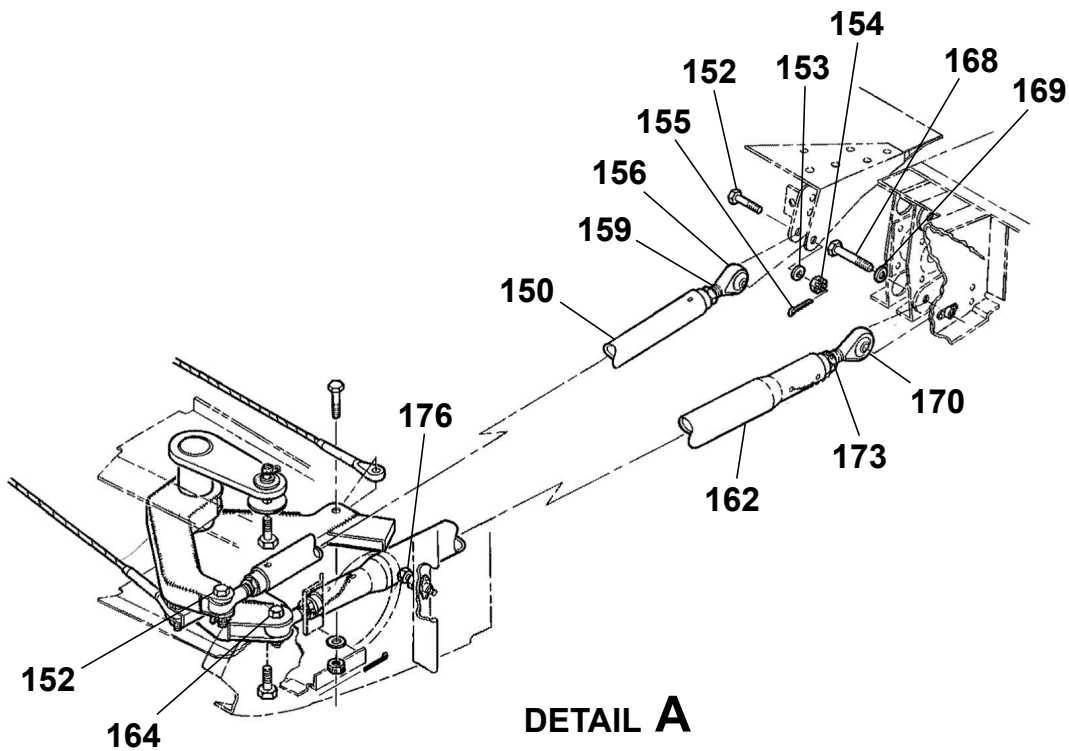
AILERON AND SPOILER CONTROL SYSTEM Figure 01. (Sheet 3)
