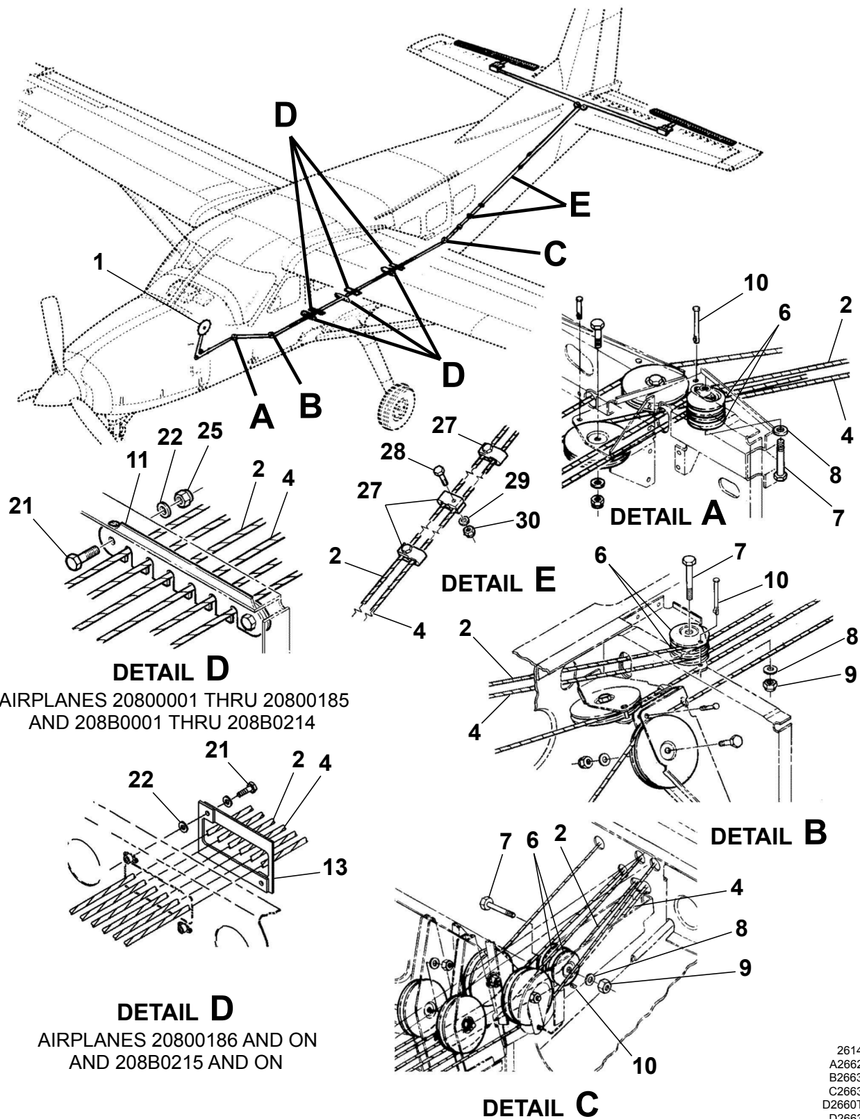
ELEVATOR TRIM CONTROL SYSTEM Figure 01. (Sheet 1)
