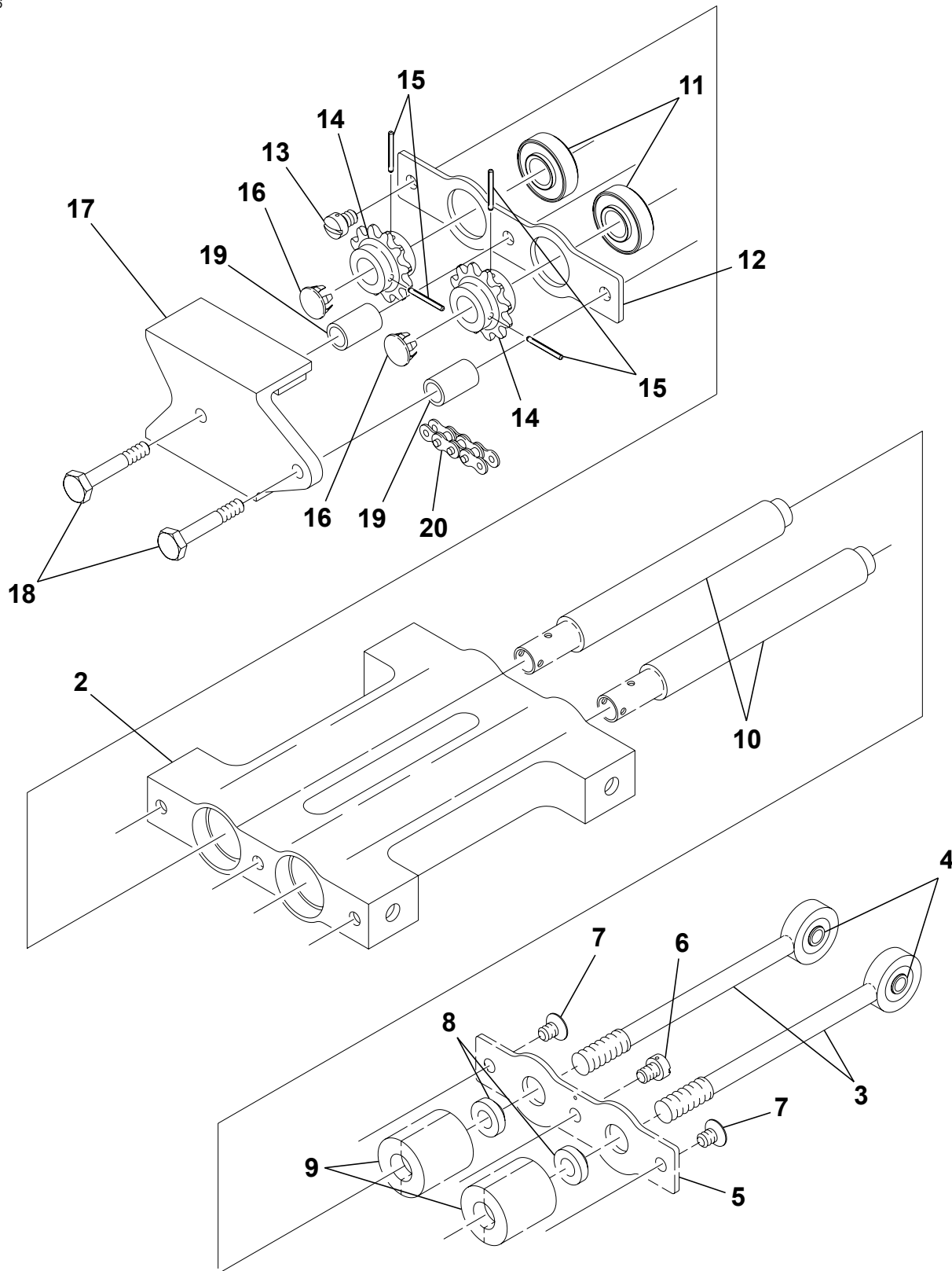
ELEVATOR TRIM TAB ACTUATOR ASSEMBLY Figure 04. (Sheet 1)
