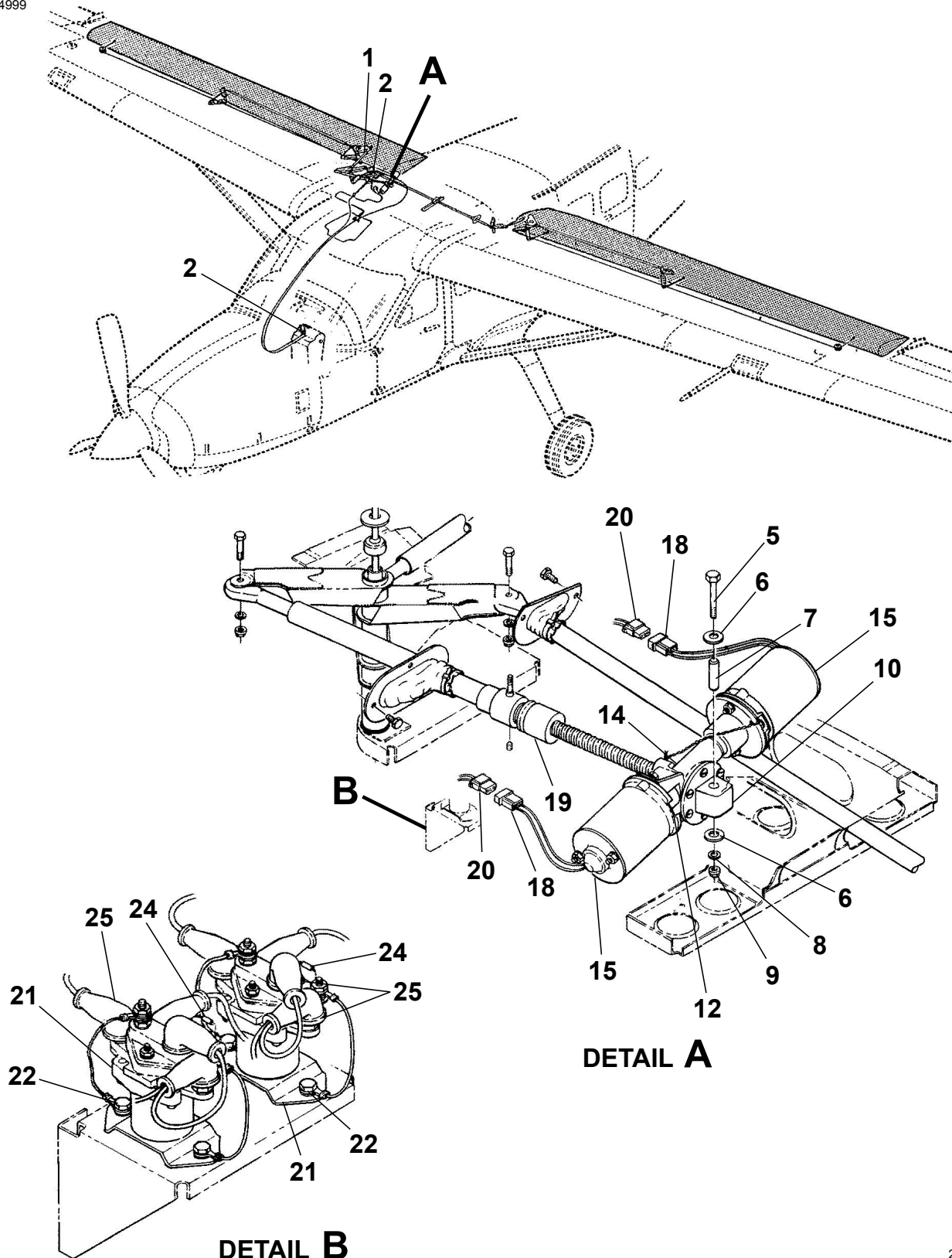
FLAP CONTROL SYSTEM Figure 01. (Sheet 1)
