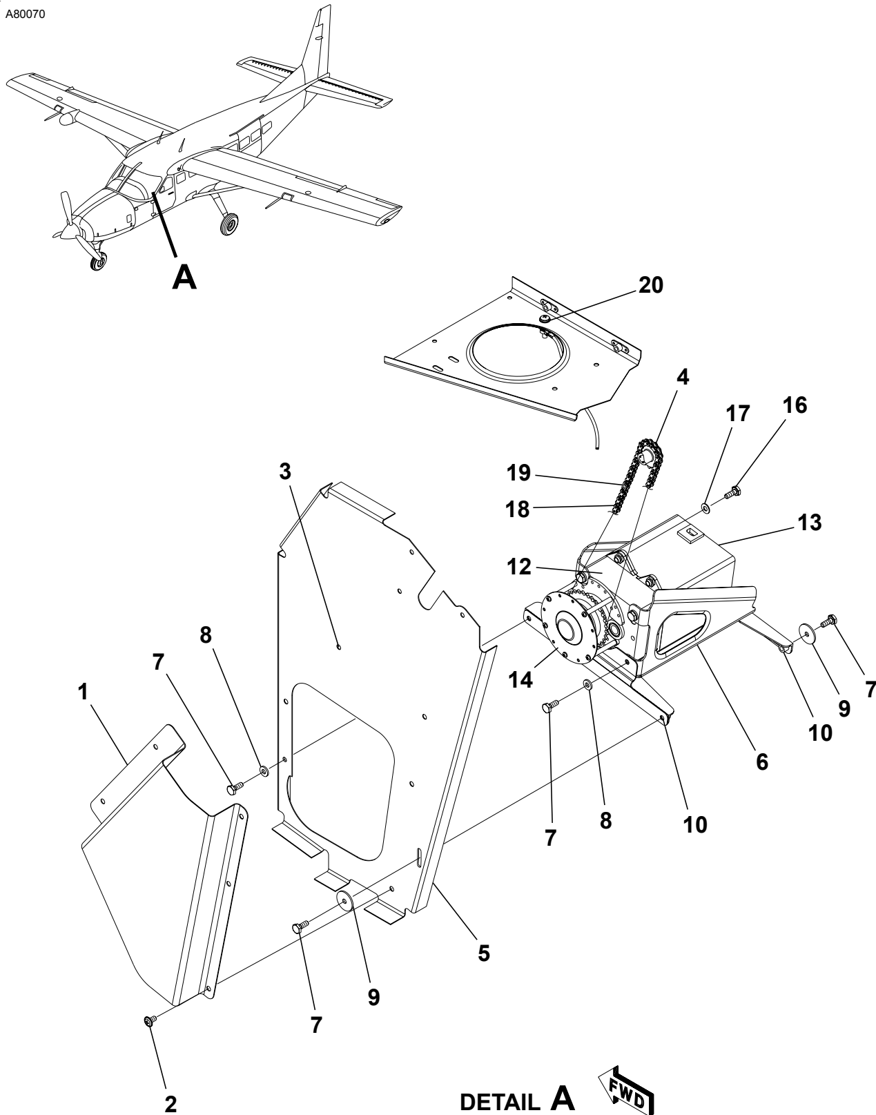
PITCH TRIM SERVO INSTALLATION Figure 02A. (Sheet 1)
