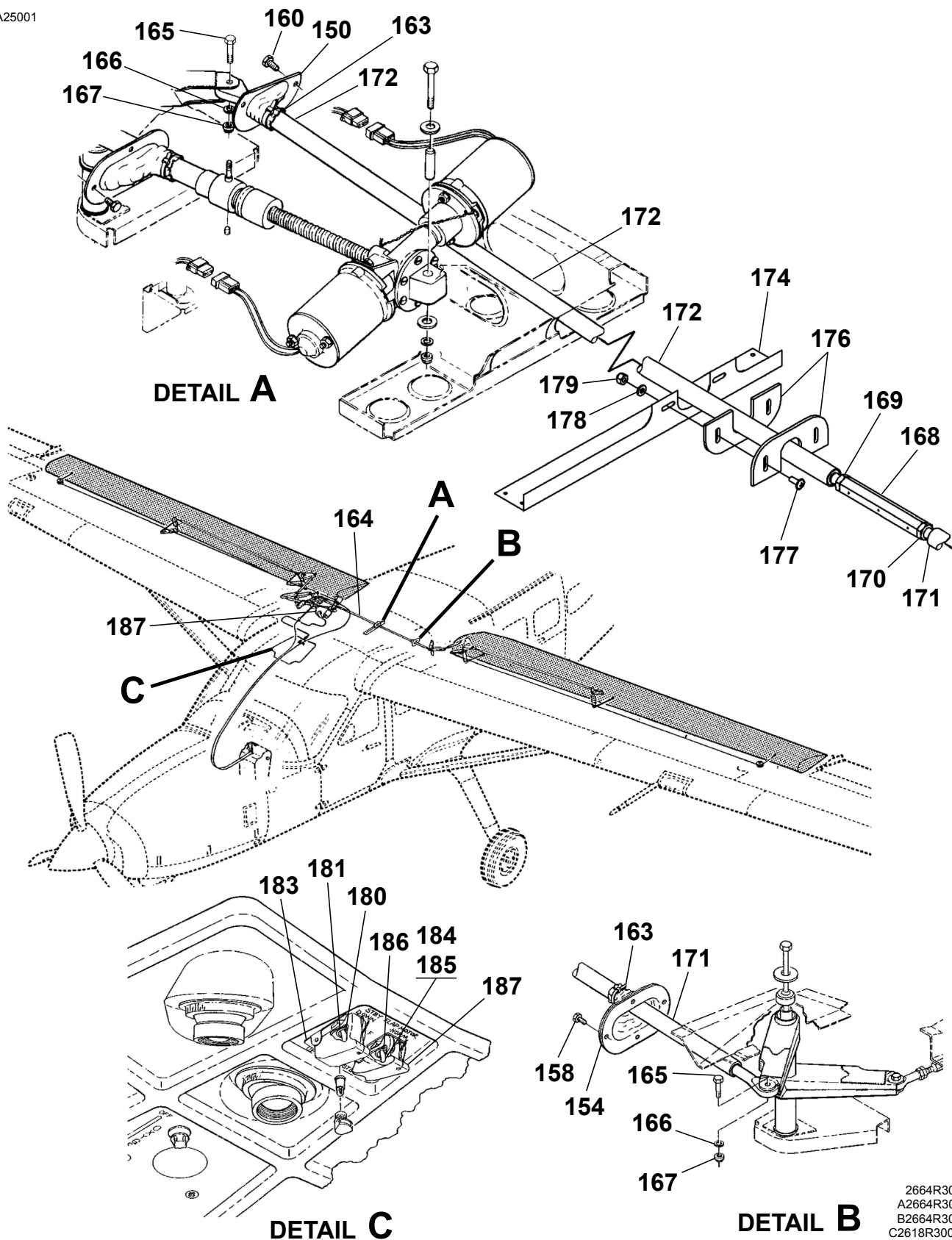
FLAP CONTROL SYSTEM Figure 01. (Sheet 3)
