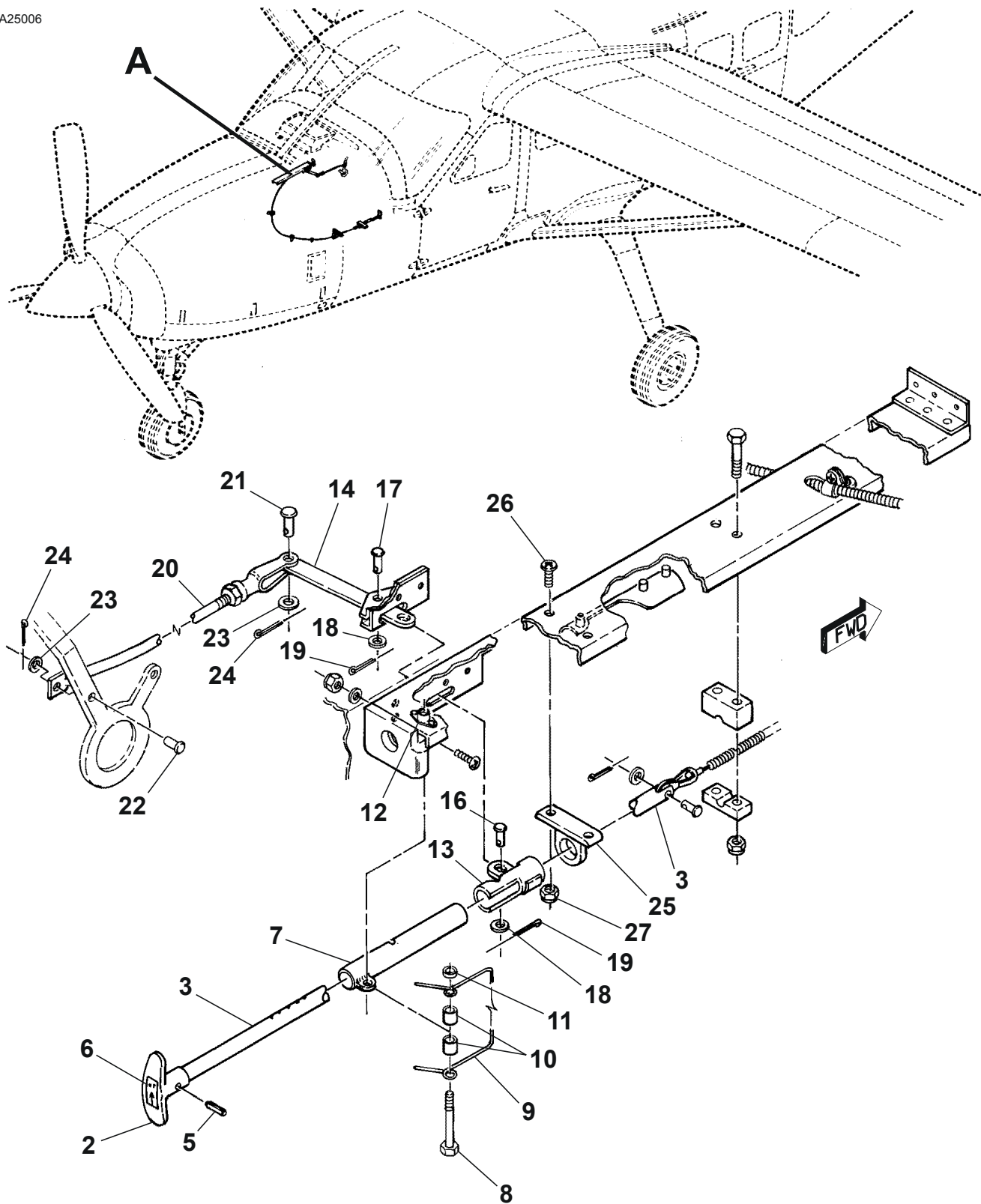
RUDDER CONTROL LOCK INSTALLATION Figure 01. (Sheet 1)
